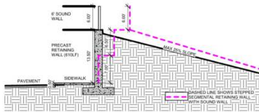
1 SOUTH BERM - LOOKING EAST 1/8" = 1'-0"
