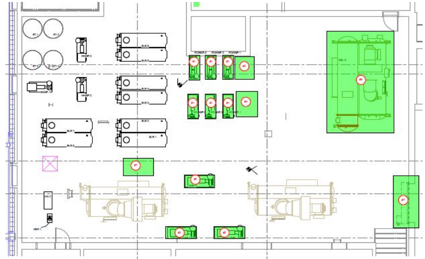
NEW CHILLER SCOPE - DRAFT
